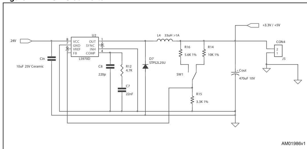
Figure 2. DC-DC converter
