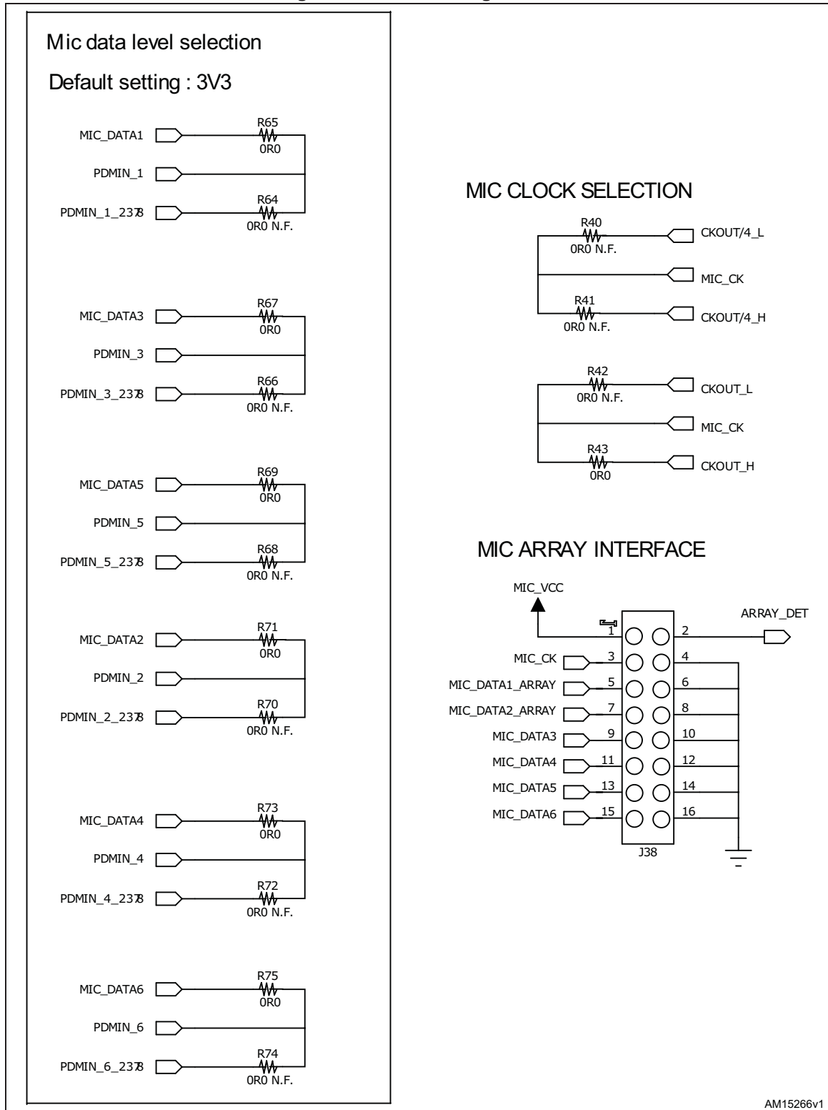
Figure 6. Schematic diagram 5/5
