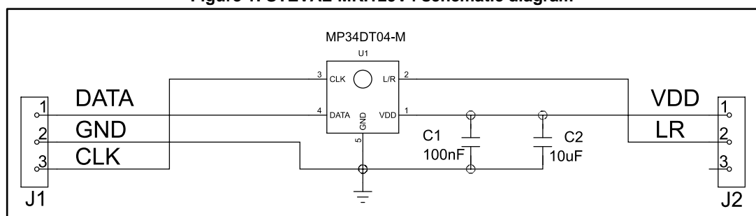
Figure 1: STEVAL-MKI129V4 schematic diagram
