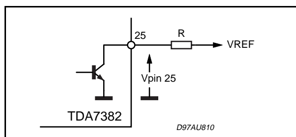
Figure 12: Diagnostics circuit.
