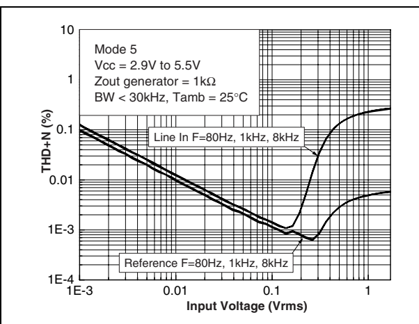
Figure 47. THD+N vs. input voltage. Line in mode 5
