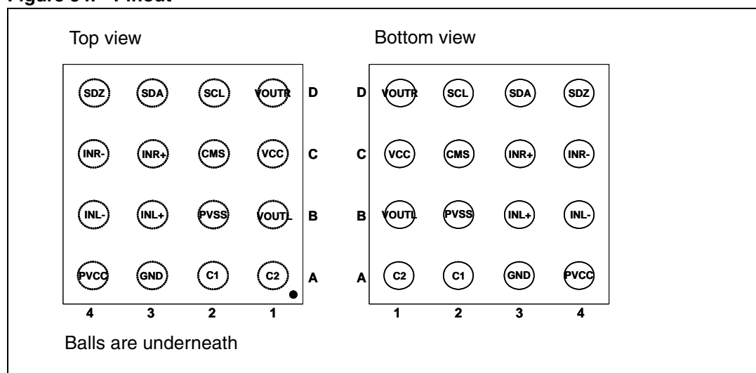
Figure 54. Pinout
