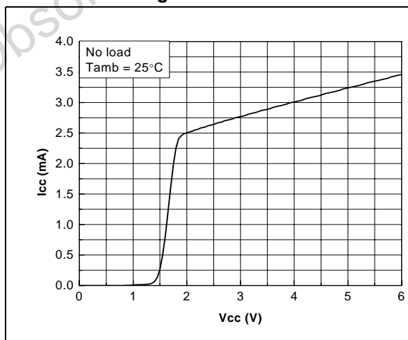
Figure 30. Current consumption vs. supply voltage
