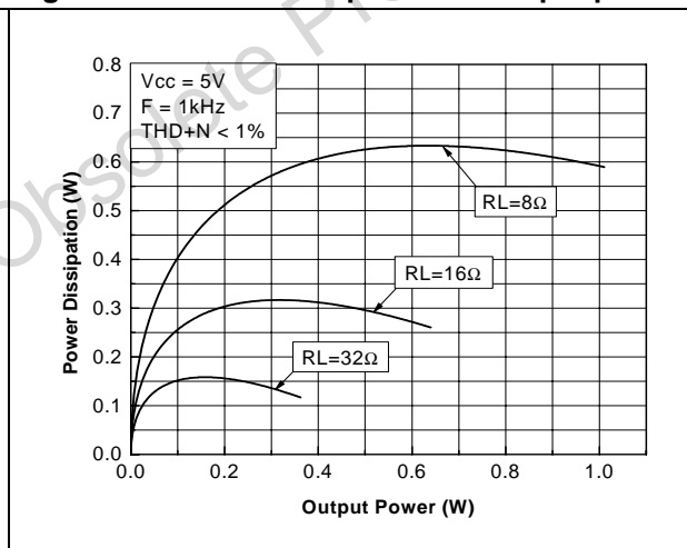
Figure 36. Power dissipation vs. output power
