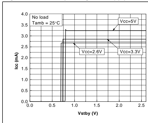
Figure 32. Standby voltage vs. supply current
