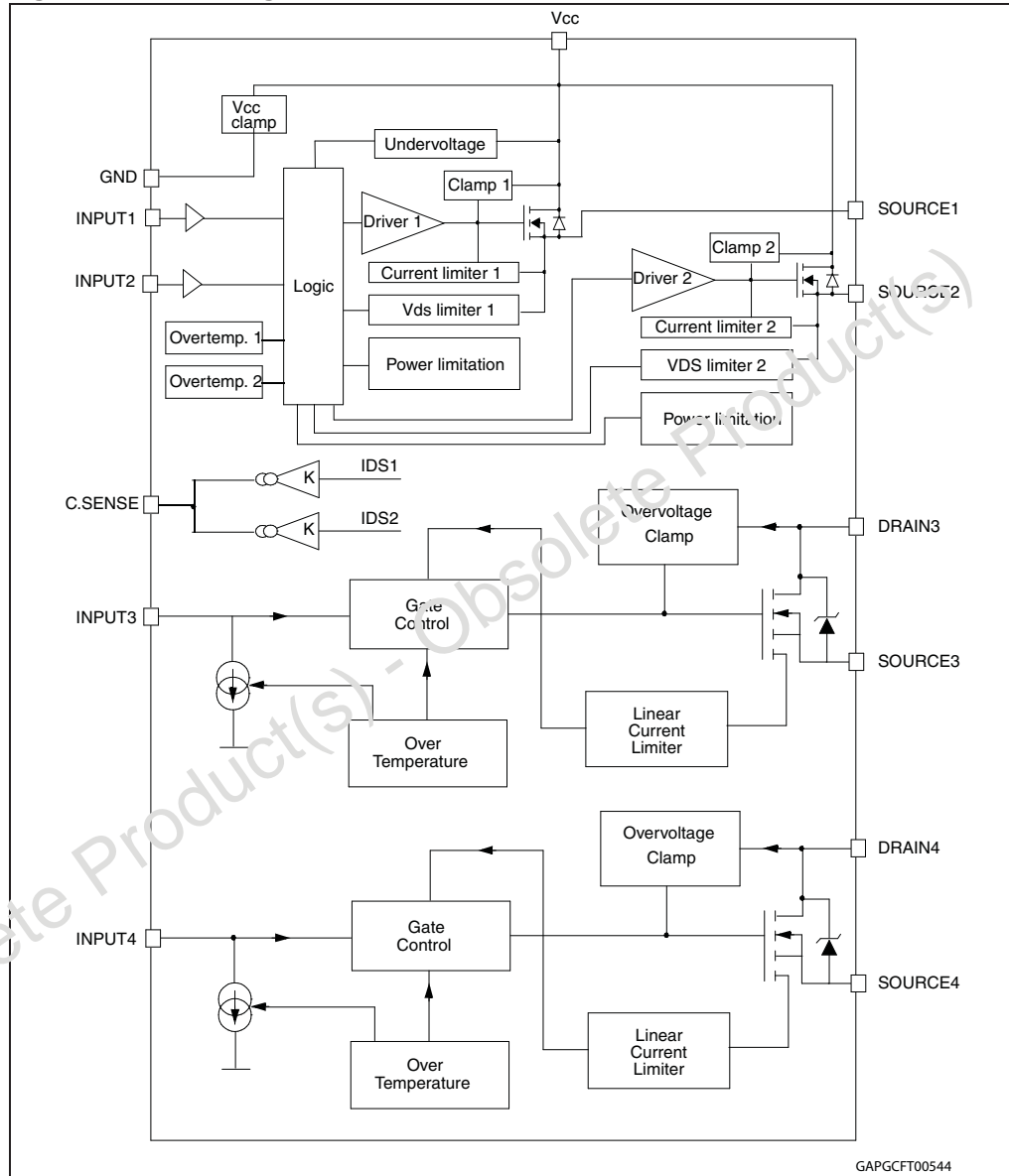
Figure 1. Block diagram
