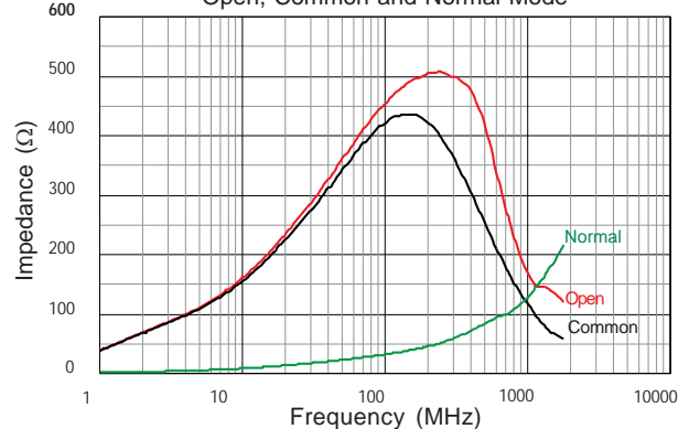
CM4545Z131B&R-00 (2 Turn) Z vs. Frequency Open, Common and Normal Mode
