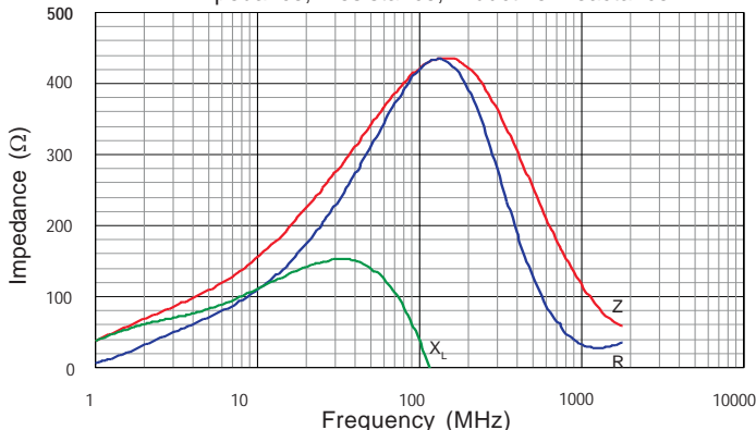
CM4545Z131B&R-00 (2 Turn) Z, R, X L vs. Frequency Impedance, Resistance, Inductive Reactance
