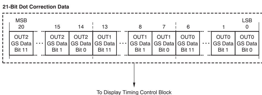
Figure 28. Dot Correction Data Latch Bit Assignment
