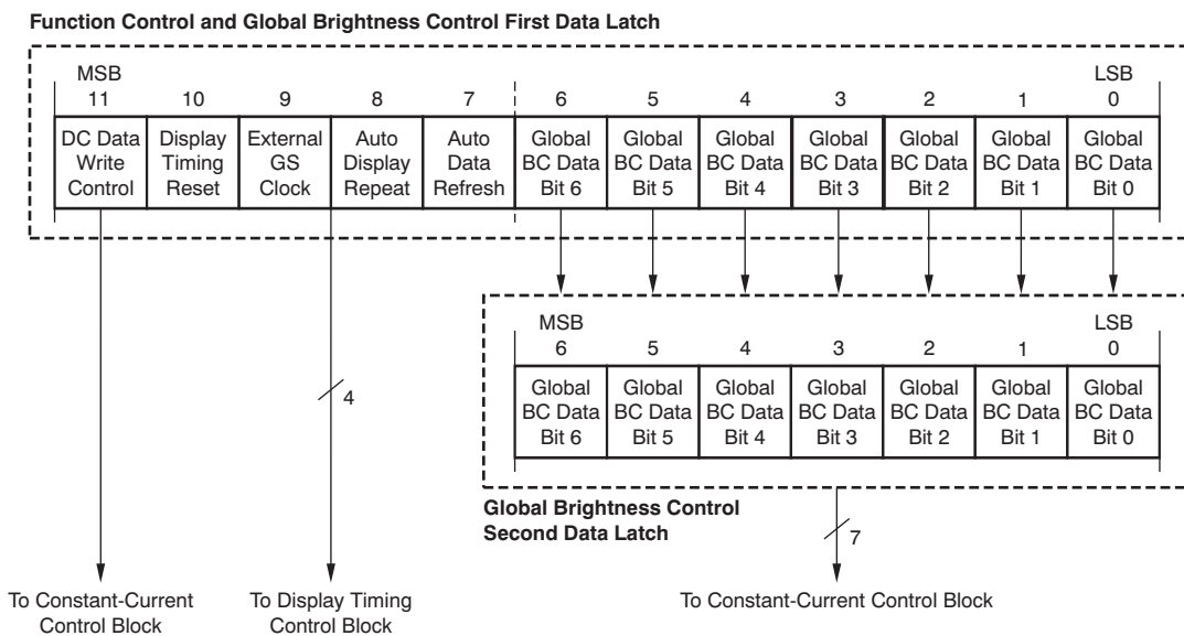
Figure 27. Function Control Data Latch Bit Assignment
