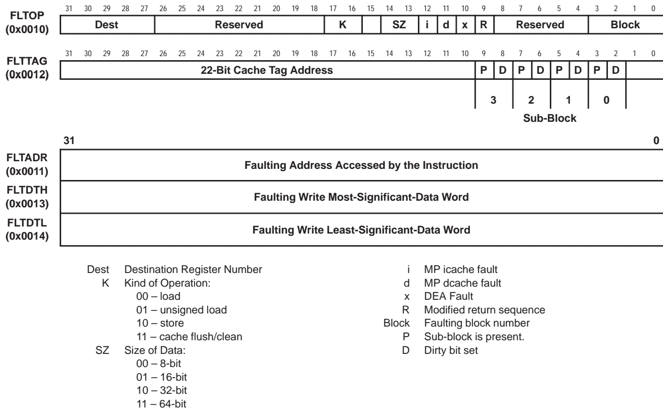
Figure 16. Memory-Fault Registers
