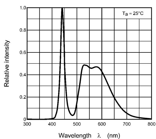
Fig. 8.6 Wavelength Characteristic
