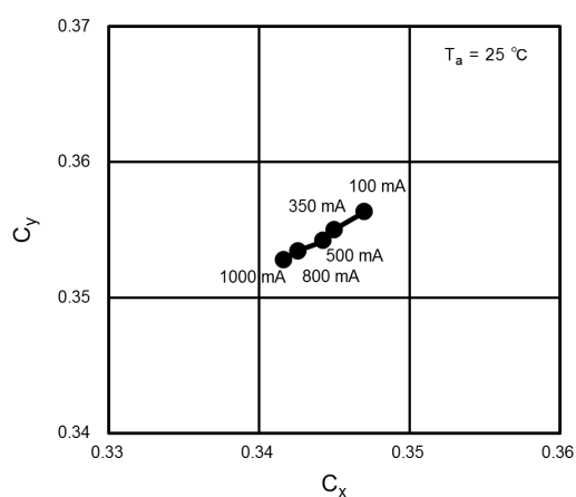
Fig. 8.4 Chromaticity - I_F
