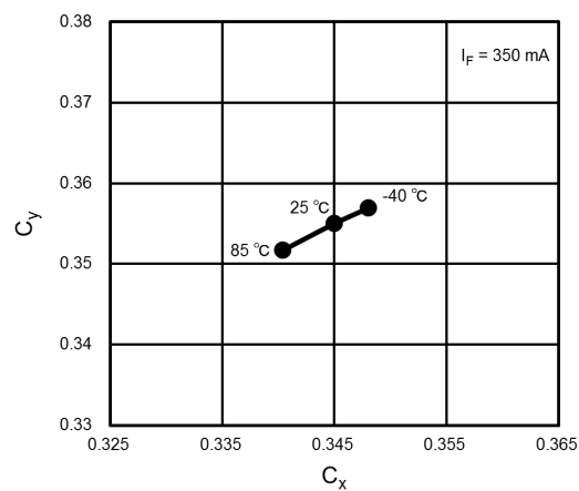
Fig. 8.5 Chromaticity - T_a
