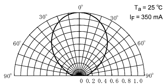
Fig. 8.7 Radiation Pattern
