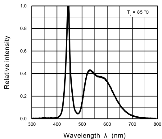
Fig. 8.7 Wavelength Characteristic
