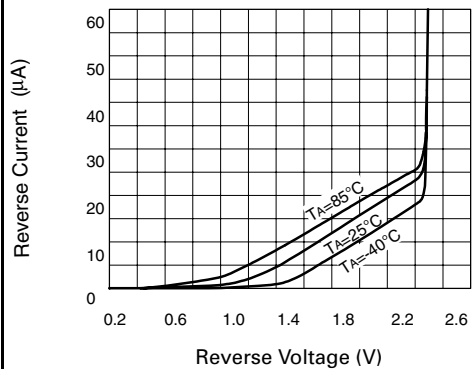
Reverse Characteristics
