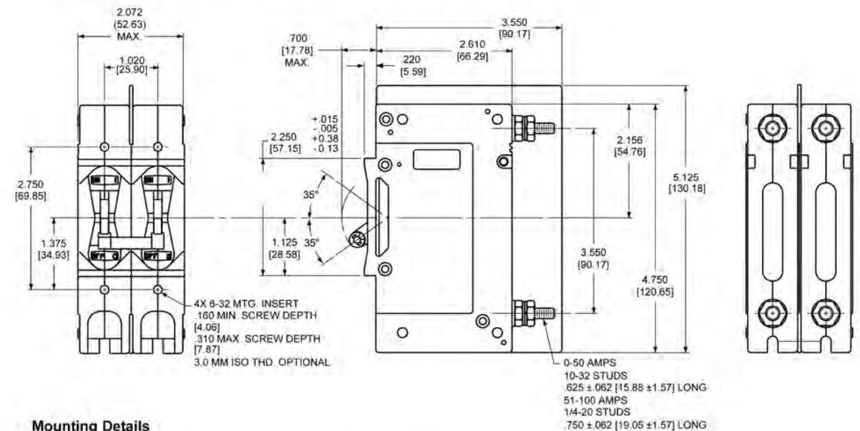
Mounting Details
