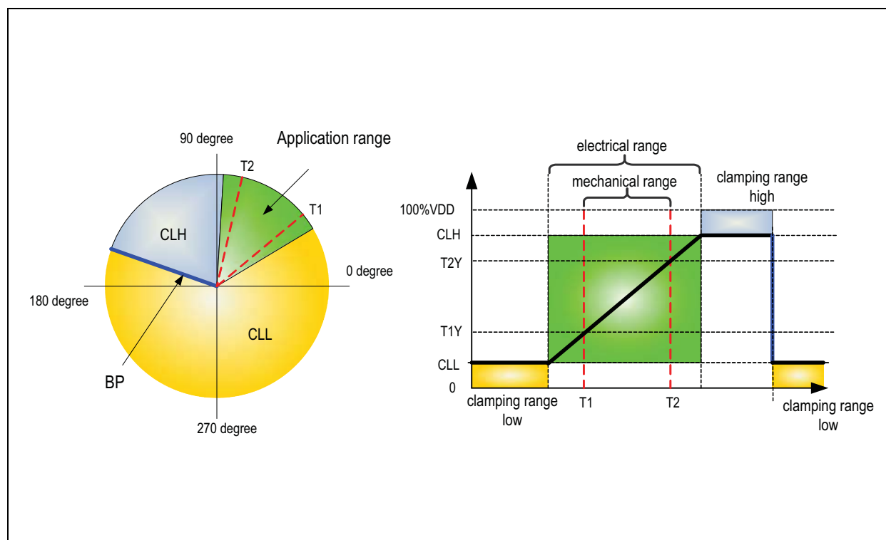
Figure 14: Individual Programming of the Break Point BP
