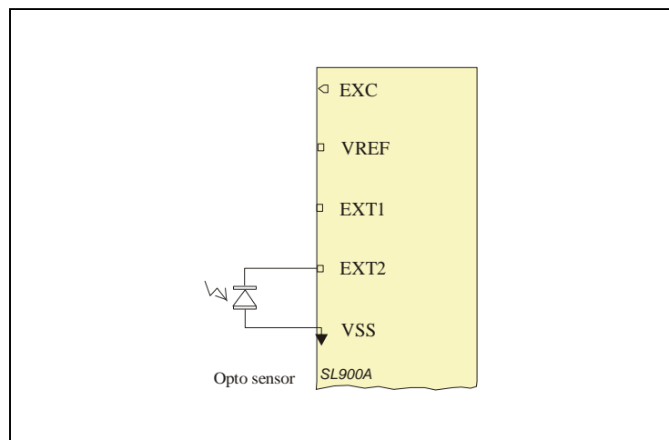
Figure 54: External Optical Sensor (EXT2 = 0)
