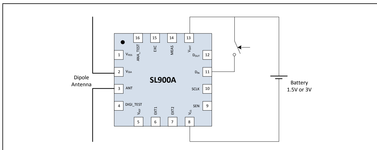
Figure 69: Battery-Assisted Transponder with Pushbutton for Manual Delayed Log Start
