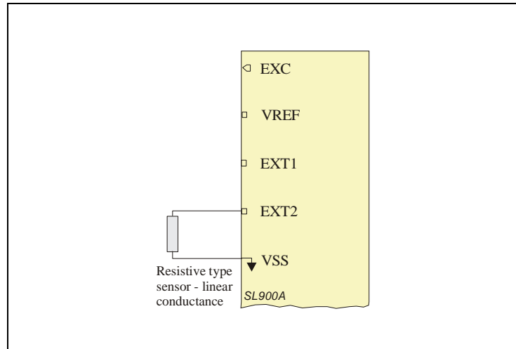
Figure 53: External Resistive Sensor - Linear Conductance (EXT2 = 0)
