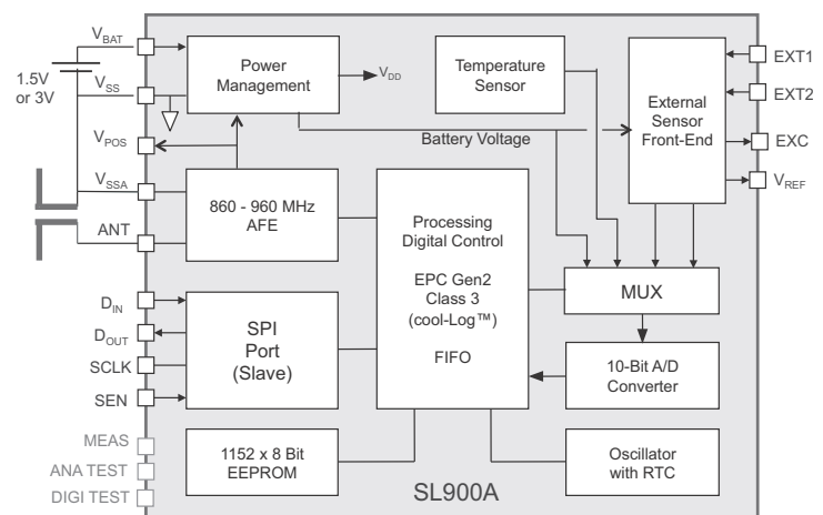
Figure 12: Block Diagram
