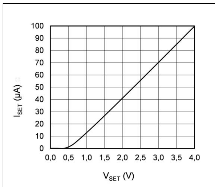
Figure 9: SET Current vs. SET Voltage, R_{SET} = 30k\Omega
