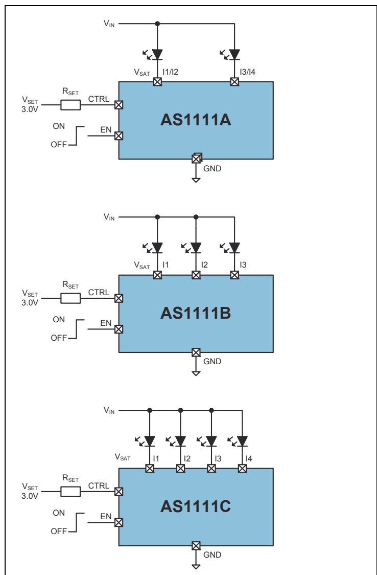
Figure 2: AS1111 Typical Application Diagram
