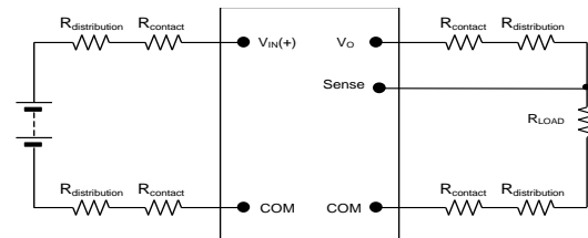
Figure 31. Remote sense circuit configuration.
