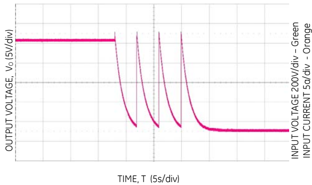
Figure 3. Overtolerance shutdown
