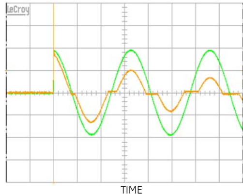
Figure 4. Inrush performance 5ms/div.
