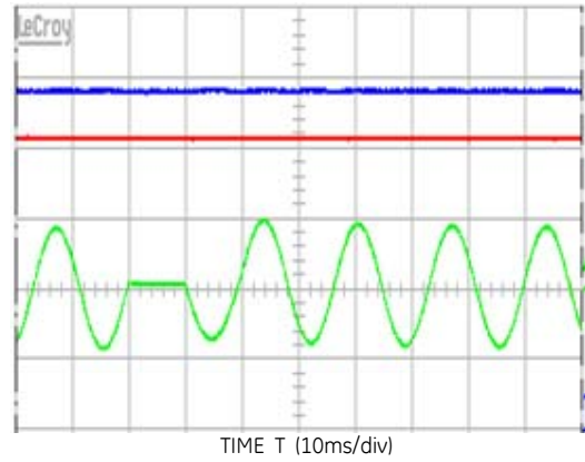
Figure 8. \frac{1}{2} cycle ride-through V_{IN} = 140V_{AC}
