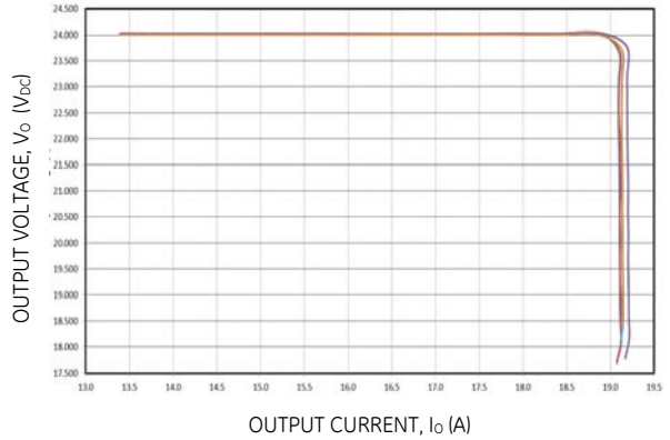
Figure 2. Output current limit profile
