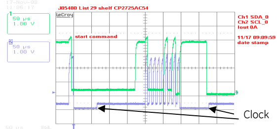
Figure 1. Example waveforms showing clock stretch
