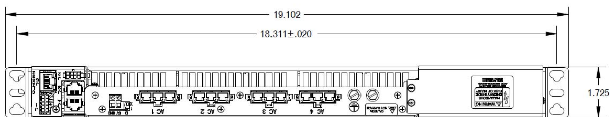
Rear View
