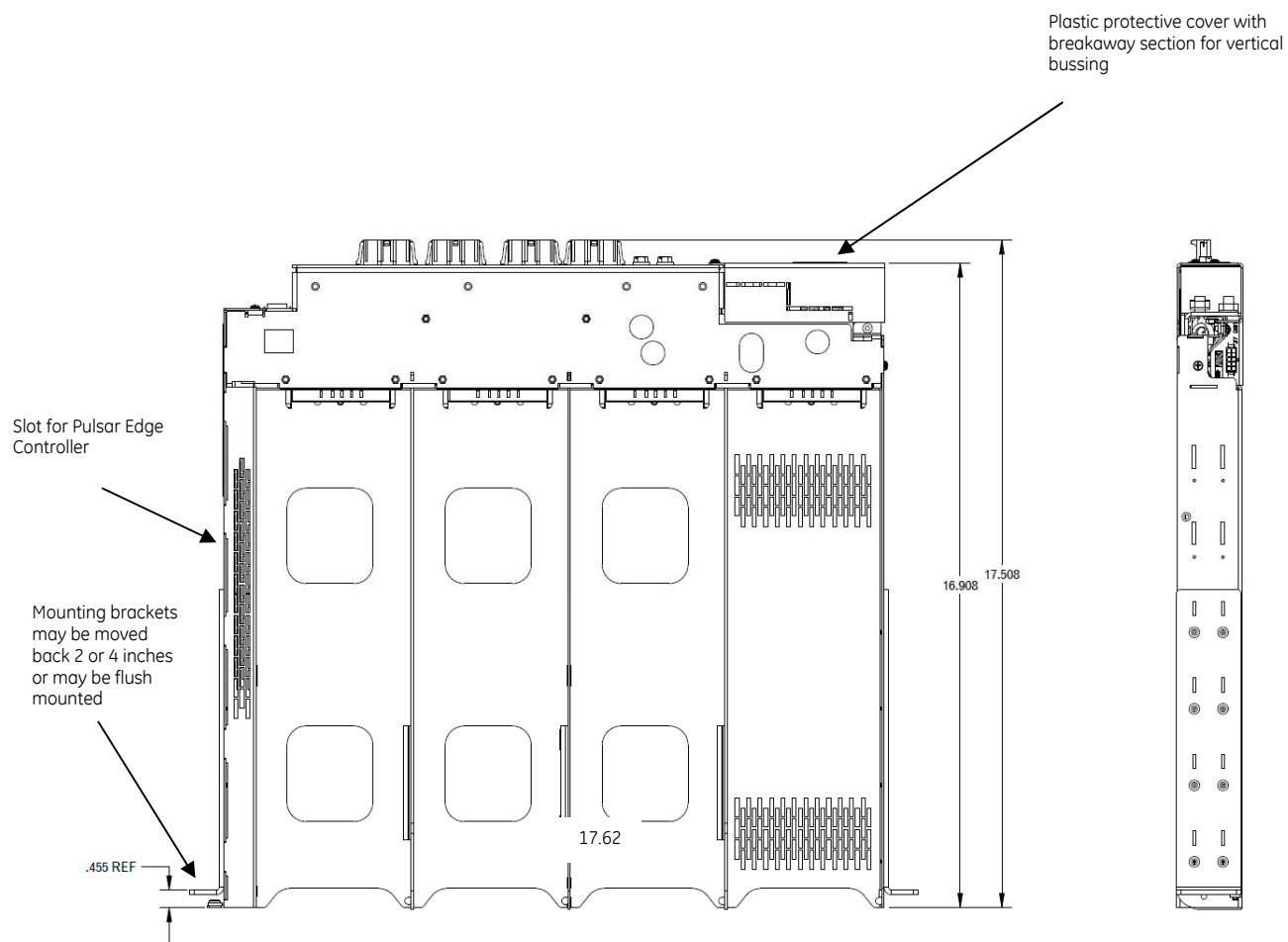
Top View
