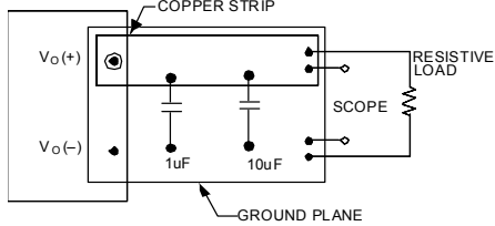
Figure 7. Input Reflected Ripple Current Test Setup.
