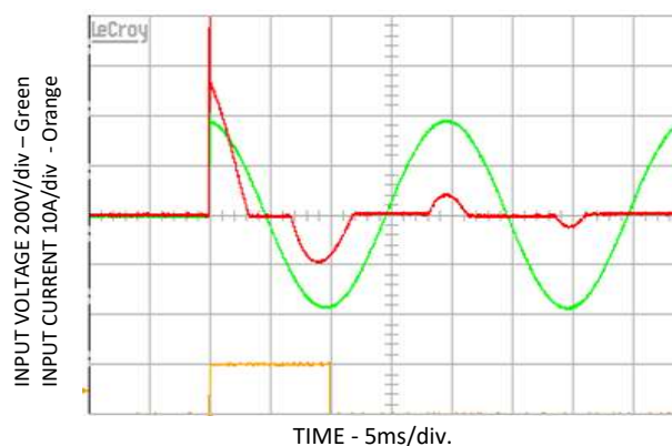
Figure 4. Inrush performance
