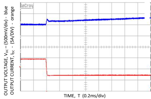
Figure 10. 54V Transient response 50% load step (100 – 50%)
