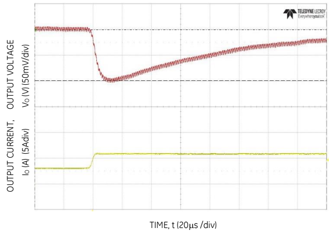
Figure 34. Transient Response to Dynamic Load Change from 50% to 100% at 12Vin, Cout=5x47µF, CTune=1800pF, RTune=300Ω
