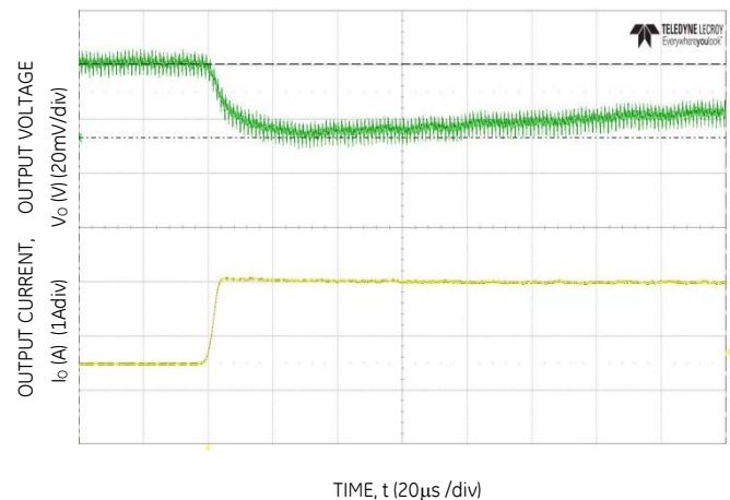
Figure 16. Transient Response to Dynamic Load Change from 50% to 100% at 12Vin, C_{out}=4 \times 47\mu\text{F} + 1 \times 330\mu\text{F} , C_{Tune}=15\text{nF} , R_{Tune}=300
