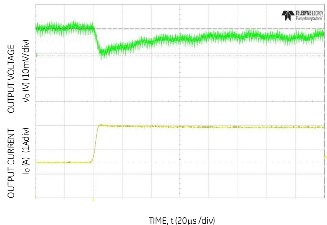
Figure 10. Transient Response to Dynamic Load Change from 50% to 100% at 12Vin, C_{out}=6 \times 47 \mu F + 1 \times 330 \mu F , C_{Tune}=5600pF , R_{Tune}=300\Omega
