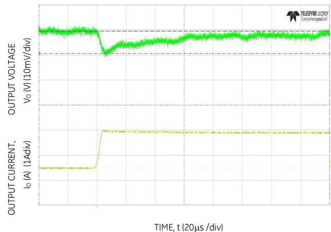
Figure 4. Transient Response to Dynamic Load Change from 50% to 100% at 12Vin, C_{out}=8 \times 47\mu F + 1 \times 330\mu F , C_{Tune}=5.6nF , R_{Tune}=300\Omega
