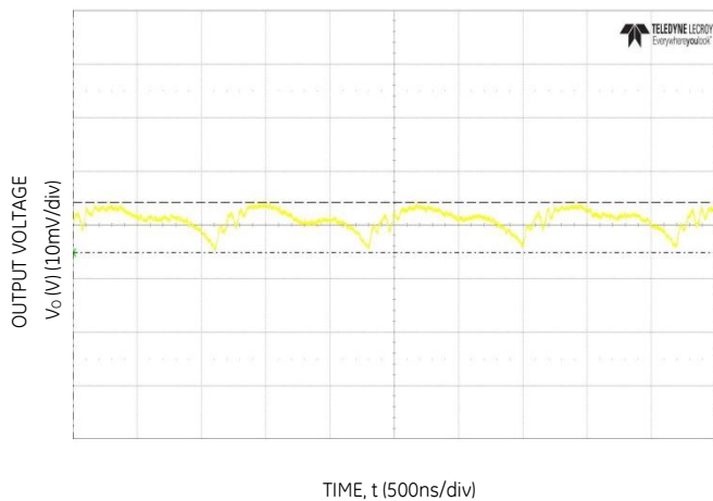
Figure 9. Typical output ripple and noise ( C_o=2 \times 47 \mu F ceramic, V_{in} = 12V , I_o = I_{o,max} ).
