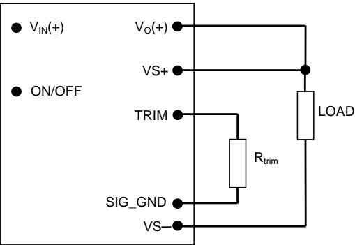
Caution – Do not connect SIG_GND to GND elsewhere in the layout Figure 42. Circuit configuration for programming output voltage using an external resistor.
