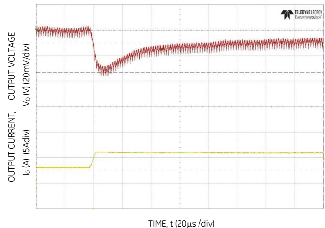
Figure 16. Transient Response to Dynamic Load Change from 50% to 100% at 12V in , C_{out}=3 \times 47 \mu\text{F} + 1 \times 330 \mu\text{F} , CT_{tune}=3900\text{pF} , RT_{tune}=300
