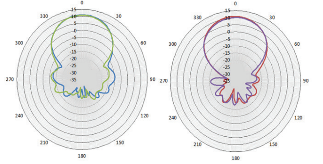
Azimuth Radiation Pattern at 2450 MHz
