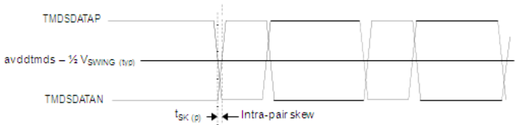
Figure 61. Intra-Pair Skew Definition
