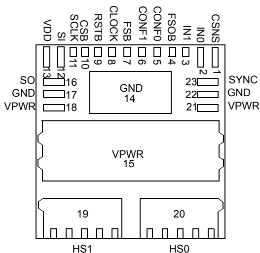
Figure 3. 20XS4200 Device Pin Assignments
