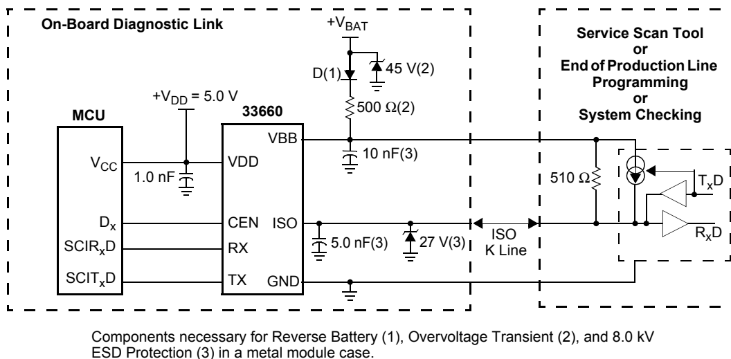
Figure 8. Typical application diagram
