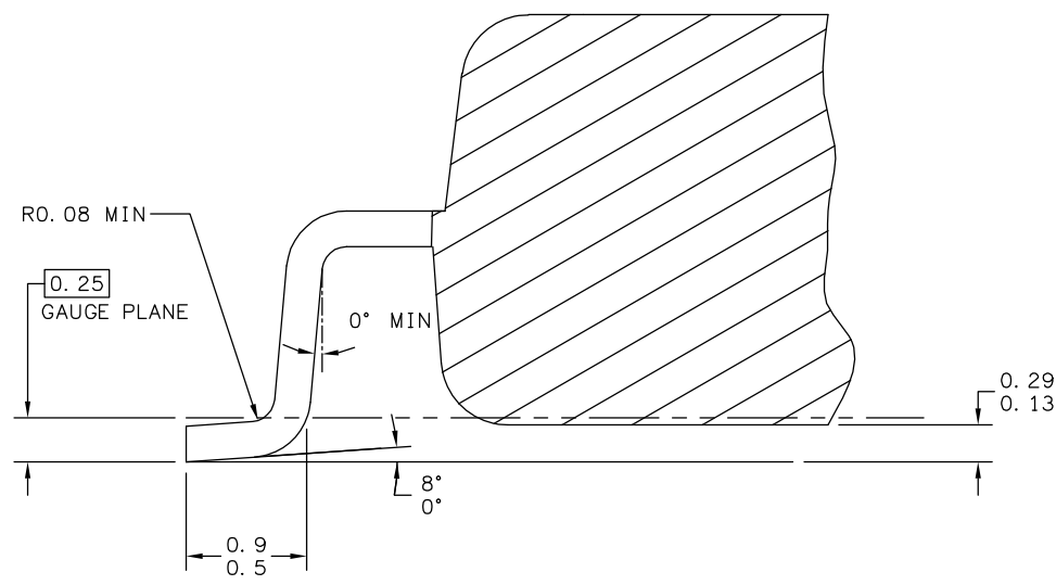
SECTION B-B
