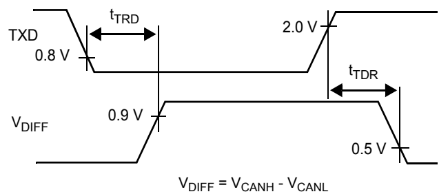
Figure 9. Propagation Delay TXD to CAN
