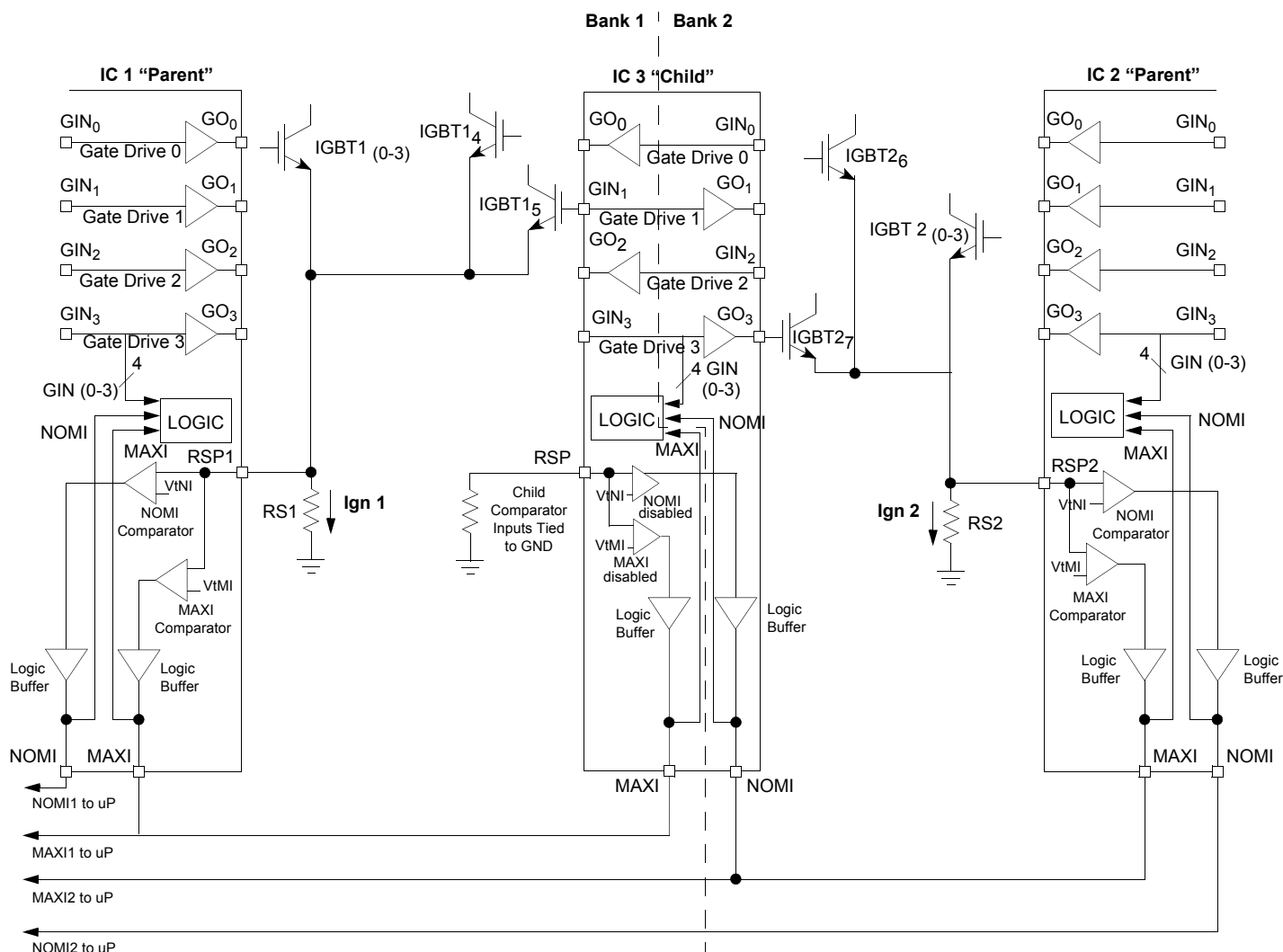
Figure 11. V10 Mode
