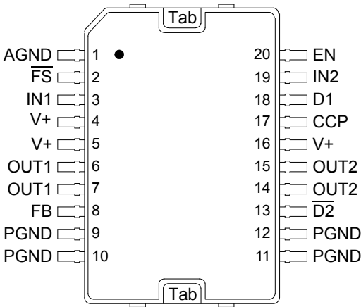
Figure 3. 33887 Pin Connections
