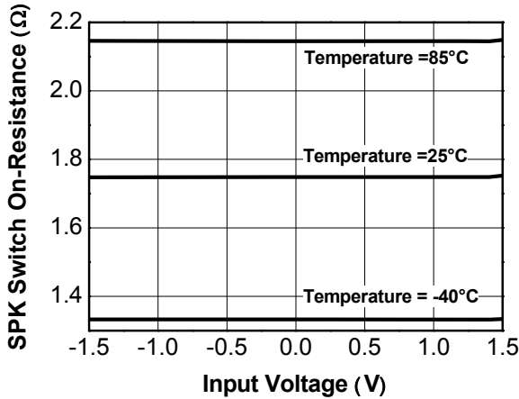
Figure 4. SPK Switch On Resistance vs Input Voltage
