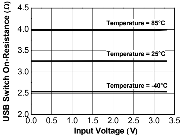
Figure 5. USB Switch On Resistance vs Input Voltage
