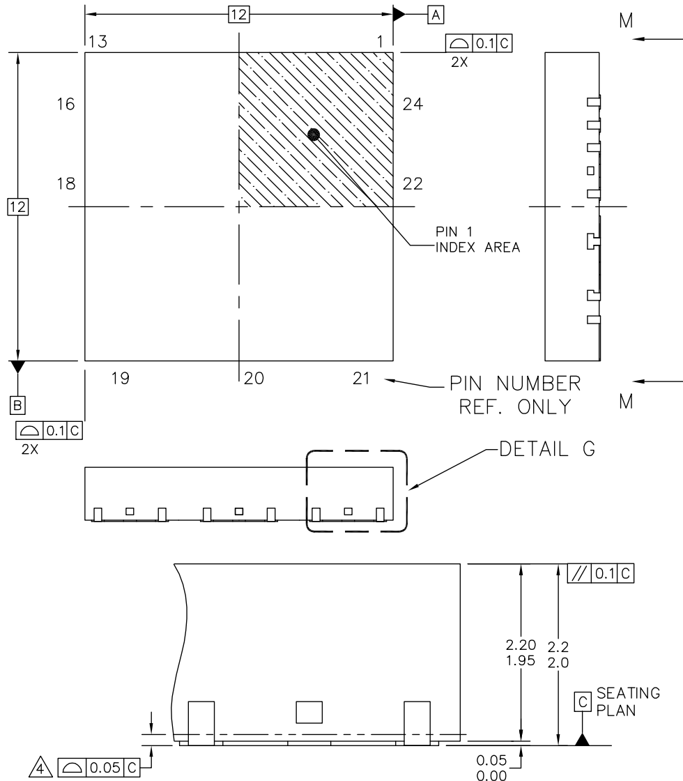
DETAIL G
