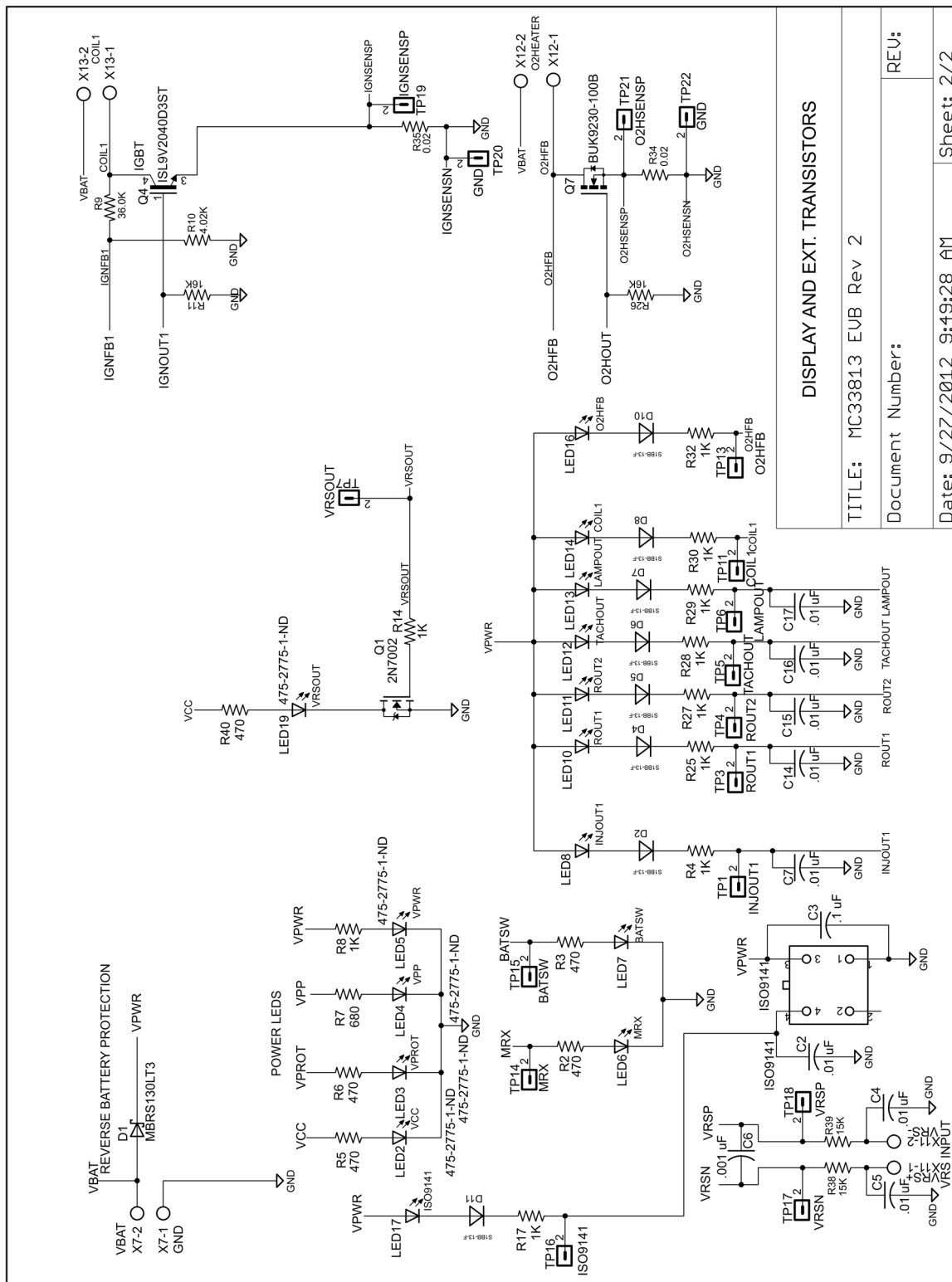
Figure 8. Evaluation Board Schematic, Part 2
