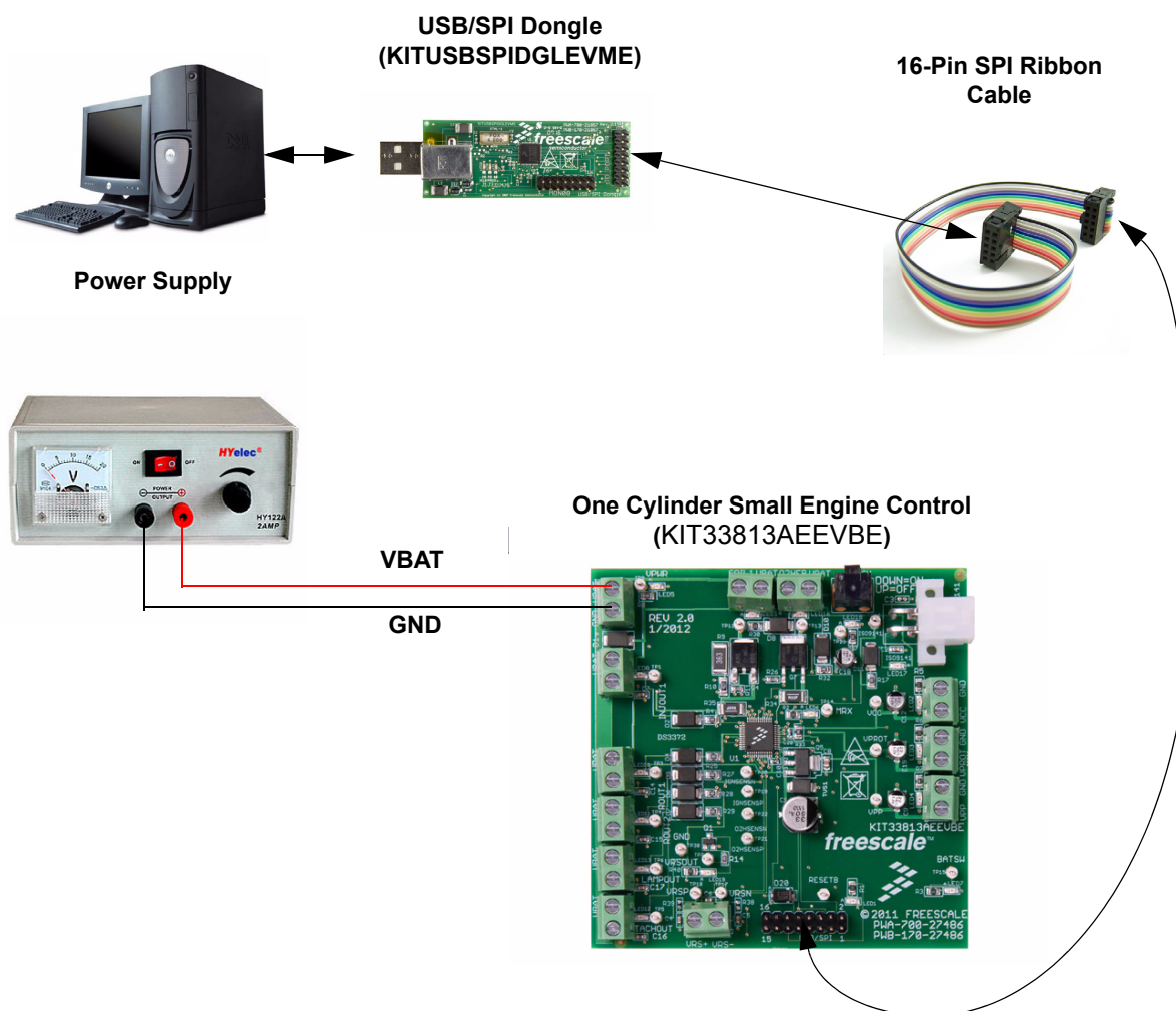
Figure 2. KIT33813AEEVBE plus KITUSBSPIDGLEVME Board Setup
