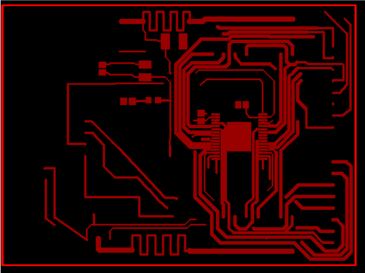
Figure 11. PCB Top
