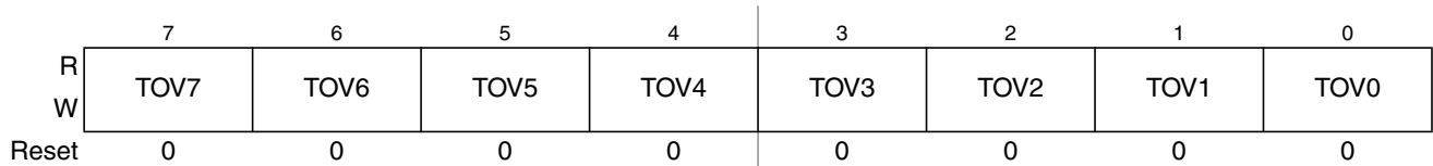
Figure 14-10. Timer Toggle On Overflow Register 1 (TTOV)
