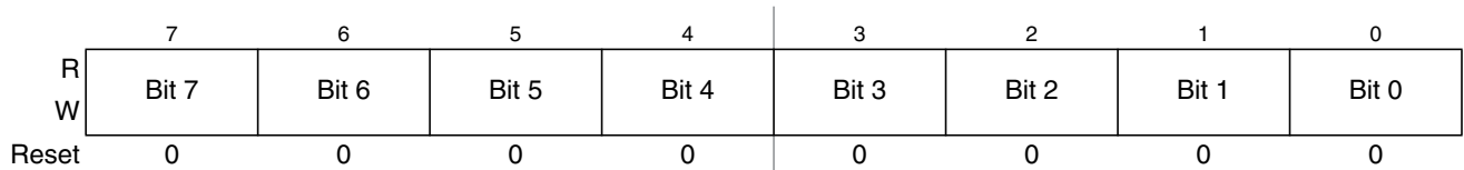
Figure 14-33. Timer Input Capture/Output Compare Register 6 Low (TC6)
