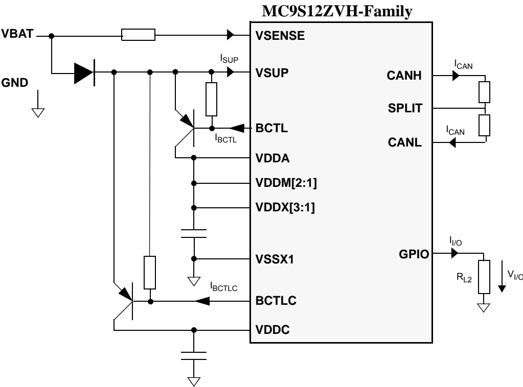
Figure A-2. Supply Currents Overview
