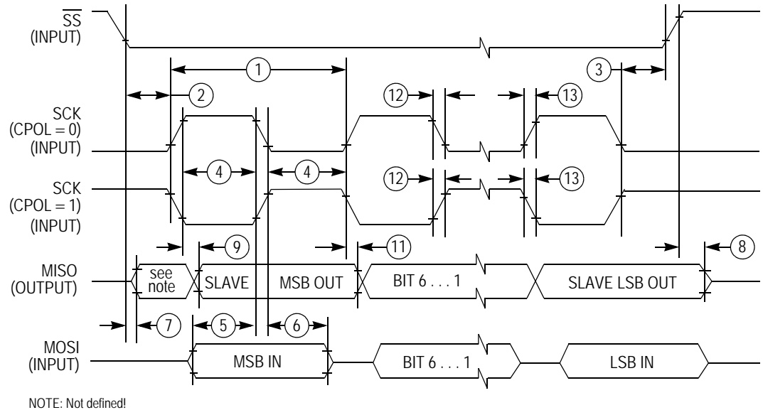
Figure M-5. SPI Slave Timing (CPHA=1)
