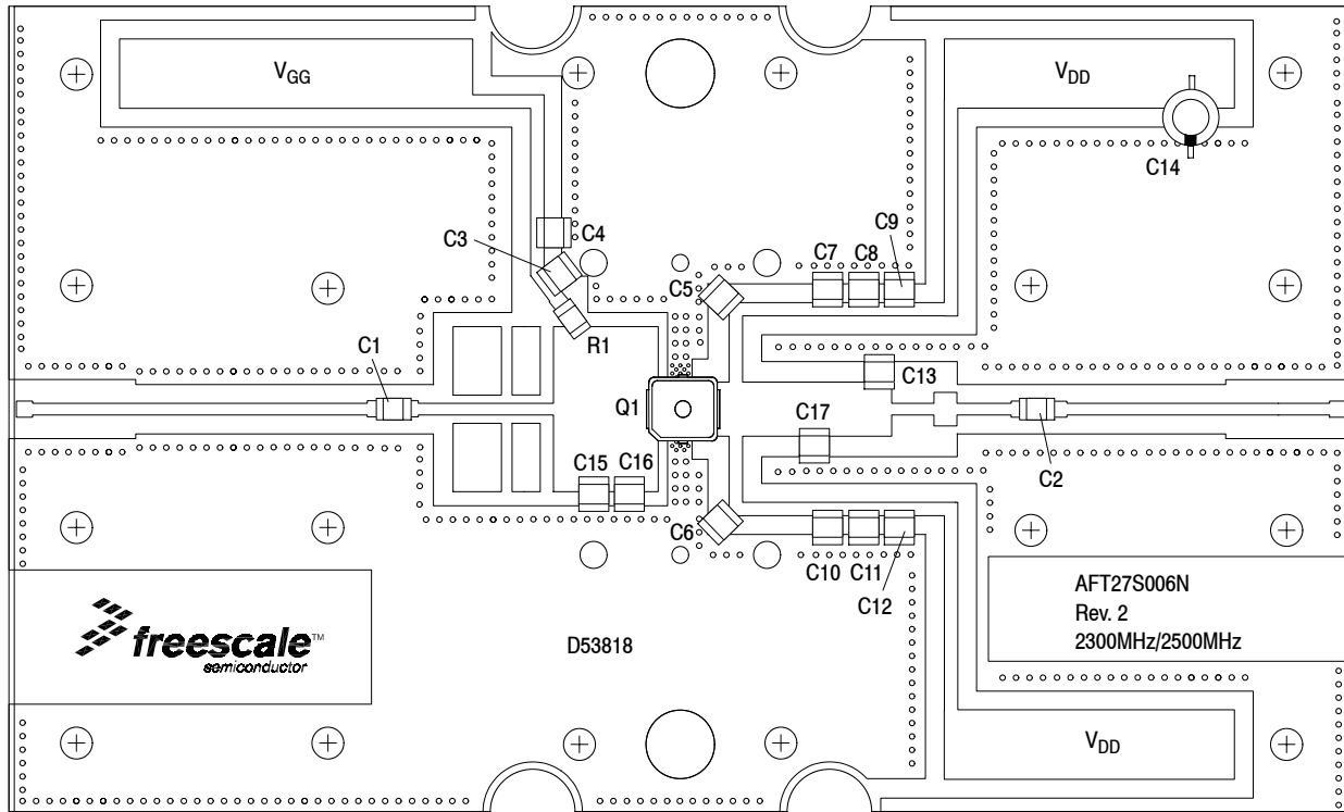
Figure 20. AFT27S006NT1 Test Circuit Component Layout — 2300-2400 MHz
