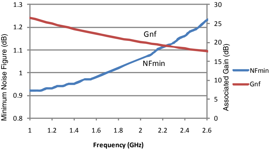
Figure 4. Minimum Noise Figure and Associated Gain vs. Frequency (R bias = 1.5 k \Omega )
