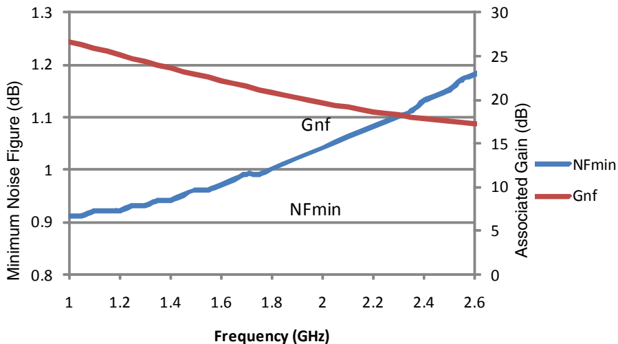
Figure 5. Minimum Noise Figure and Associated Gain vs. Frequency (R bias = 1.2 k \Omega )
