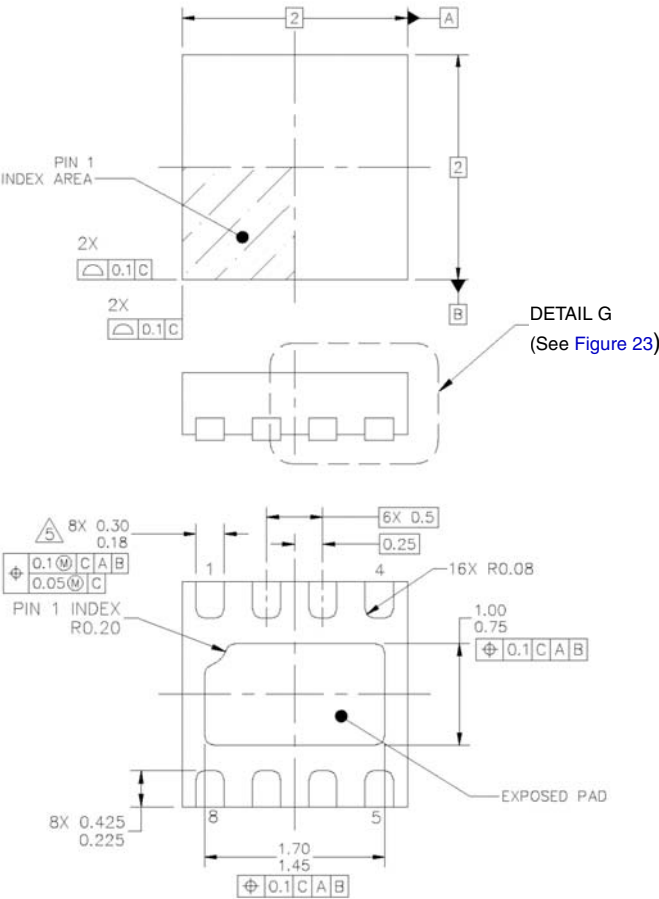
Figure 22. Outline Dimensions for MLPD-8
