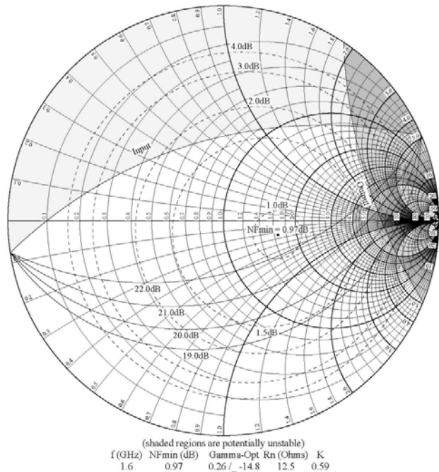
Figure 14. Constant Noise Figure and Gain Circles, 1600 MHz, Rbias=1.2 kΩ
