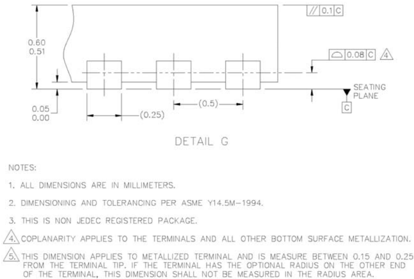
Figure 23. Package Details
