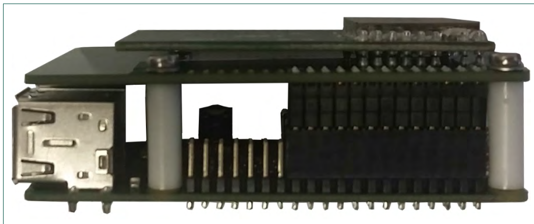
Fig 3. OM5578/PN7150RPI demo kit and Raspberry Pi stacked together
