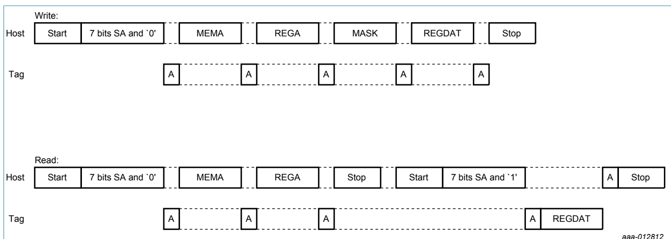
Figure 19. WRITE and READ register operation
