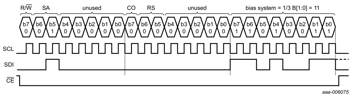
Fig 40. SPI-bus example
