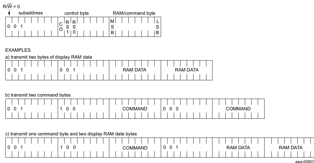
Fig 42. SPI-bus protocol - write example
