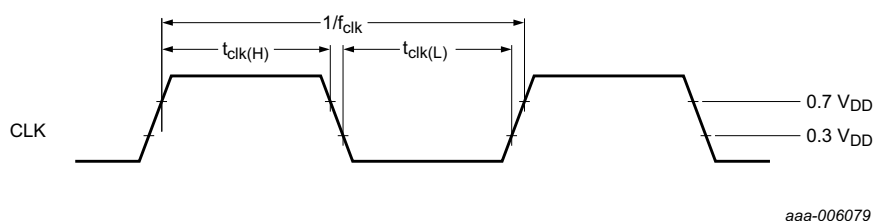
Fig 51. Driver timing waveforms
