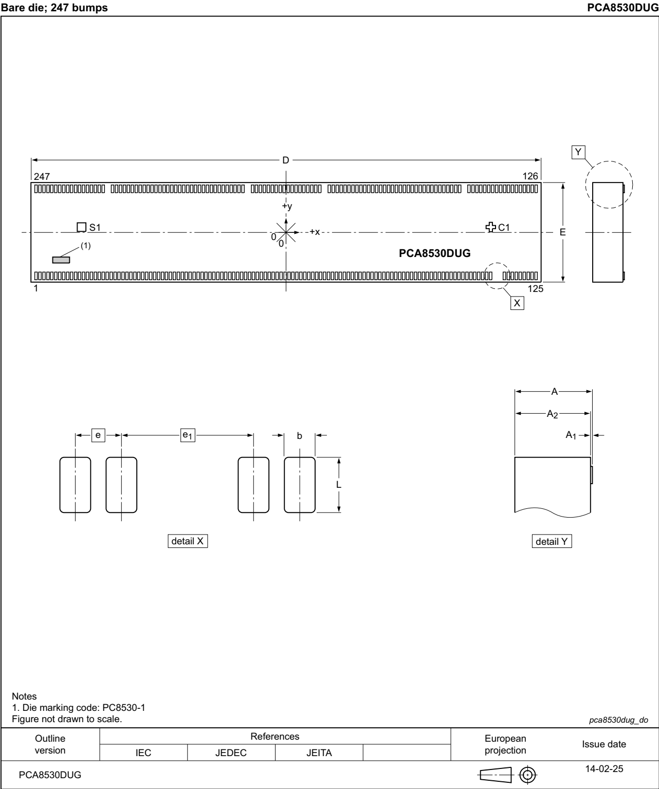
Fig 59. Bare die outline of PCA8530DUG
