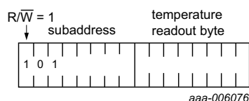
Fig 41. SPI-bus protocol - read example
