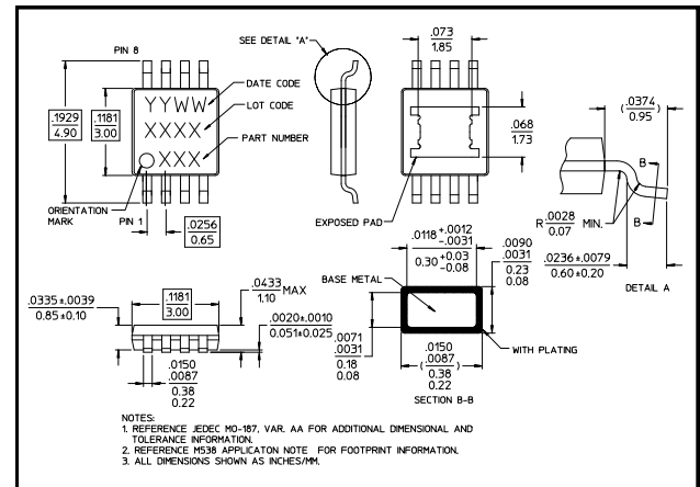
Lead-Free MSOP-8-EP†
