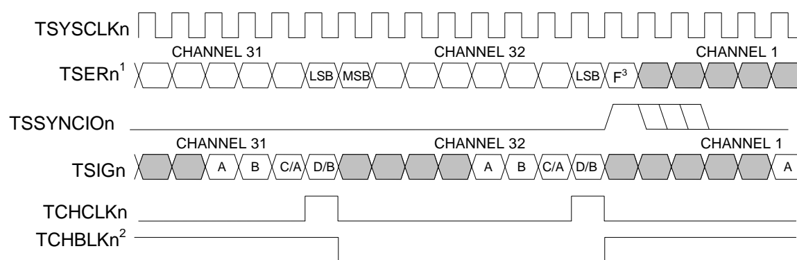
Figure 11-13. T1 Transmit-Side 2.048MHz Boundary Timing (Elastic Store Enabled)
