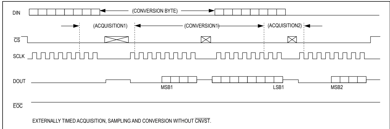
Figure 7. Clock Mode 11 Timing
