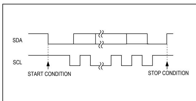
Figure 4. START and STOP Conditions
